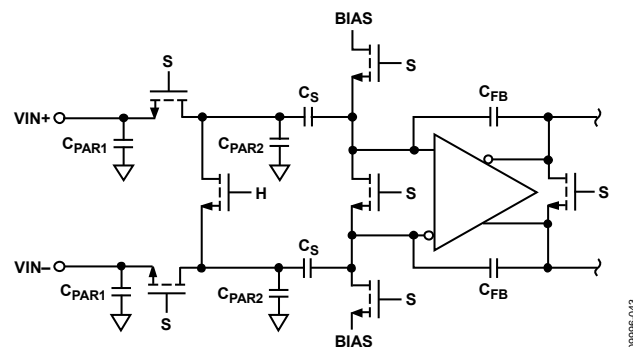
Figure 46. Switched-Capacitor Input
