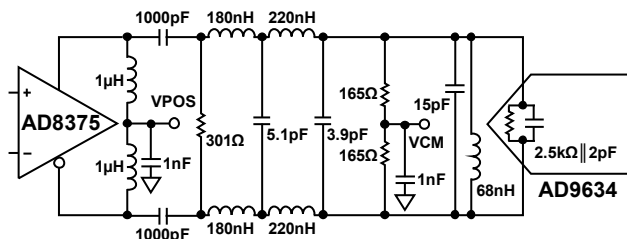
Figure 50. Differential Input Configuration Using the AD8375
