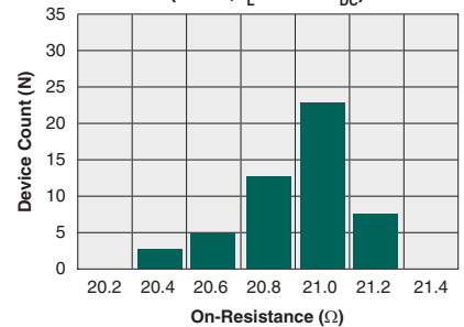
Typical On-Resistance Distribution (N=50, I_L=120mA_{DC} )
