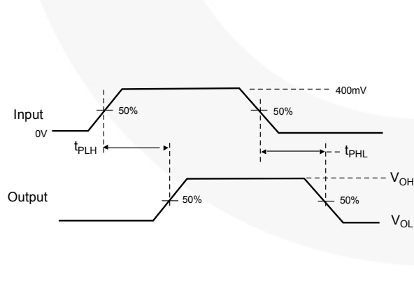
Figure 9. Propagation Delay ( t_{RtF} – 500ps)
