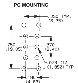
PC MOUNTING
