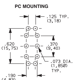
8261SH9_BE2 DPDT
