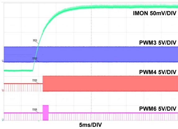
FIGURE 56. PHASE ADD TRANSITION IN BUCK/DE (3PH → 6PH → 4PH), I_O = 36A \rightarrow 110A
