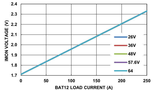
FIGURE 88. IMON vs LOAD CURRENT IN BUCK/FPWM/NO-PD WITH BAT48 VARIABLE
