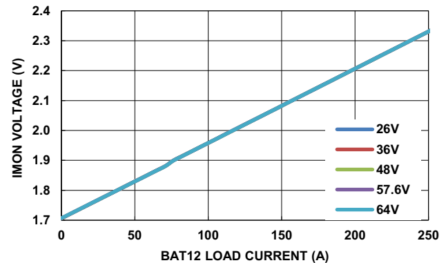
FIGURE 86. IMON vs LOAD CURRENT IN BUCK/FPWM/PD WITH BAT48 VARIABLE
