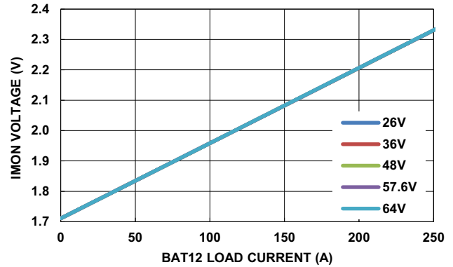
FIGURE 84. IMON vs LOAD CURRENT IN BUCK/DE/NO-PD WITH BAT48 VARIABLE
