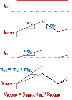
FIGURE 136. SLOPE COMPENSATION BLOCK DIAGRAM
