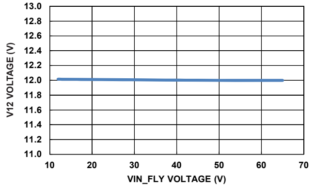
FIGURE 72. V12 LINE REGULATION, TEMP = +25°C, f SW = 100kHz, V6 LOAD = 200Ω, V12 LOAD = 200mA
