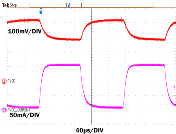
FIGURE 75. INTERNAL LDO LOAD TRANSIENT, PVCC OFFSET 4.79V, TRANSIENT LOAD 0mA TO 150mA, +25°C
