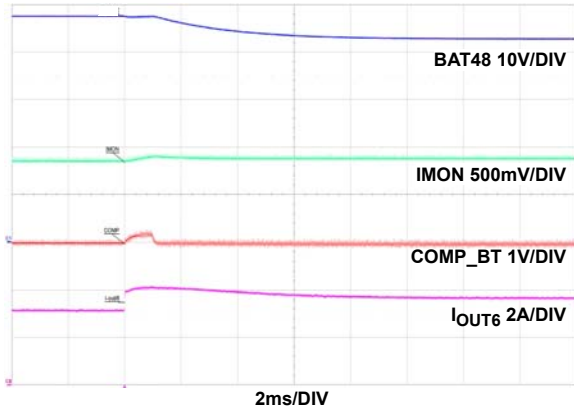
FIGURE 71. AVERAGE CONSTANT CURRENT CONTROL LOOP, CCL TRANSITION IN BOOST/DE/NO-PD, RL1 = 2.5Ω → 2Ω
