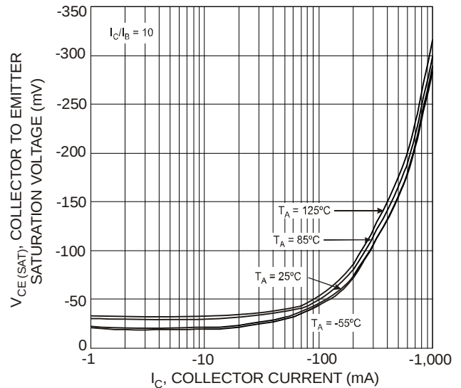
Fig. 4, Collector-Emmitter Saturation Voltage vs. Collector Current
