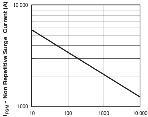
t_p - Square Wave Pulse Duration ( \mu s ) Fig. 7 - Maximum Non-Repetitive Surge Current
