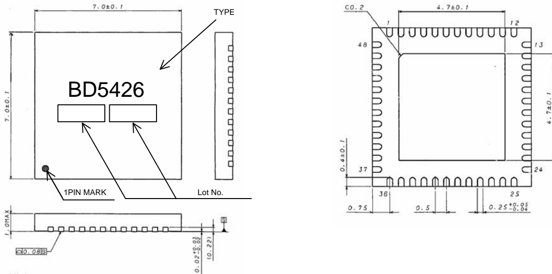
Fig. 24 Outer Dimensions and Inscriptions of VQFN048V7070 Package
