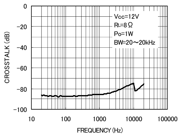
Fig. 4 Crosstalk - Frequency
