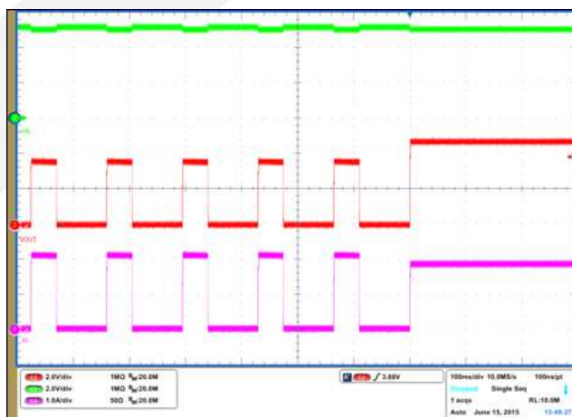
Over Current Recovery ( R_{OUT}=2.5\Omega )
