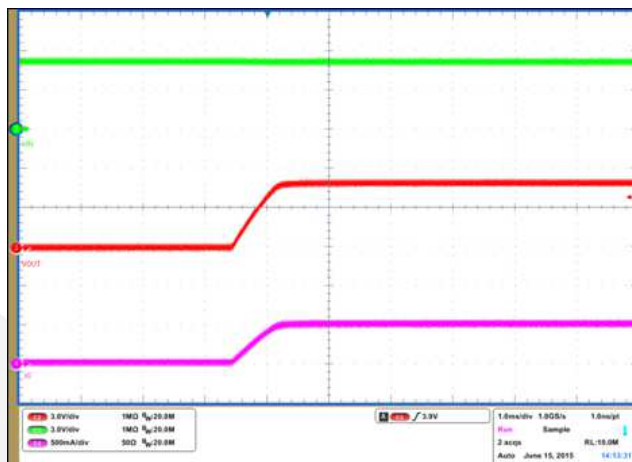
Over Temperature Recovery (R OUT =10Ω)
