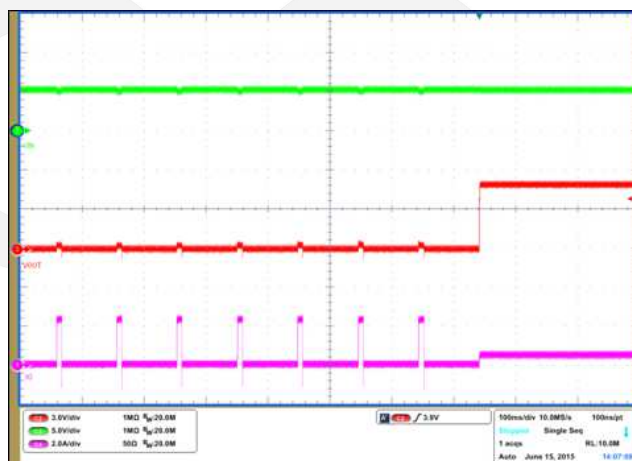
Short Circuit Recovery ( R_{OUT}=10\Omega )
