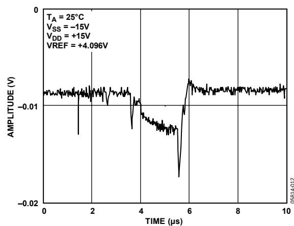
Figure 12. Analog Crosstalk Due to \overline{LDAC}
