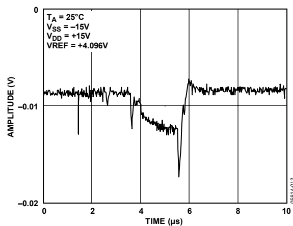
Figure 12. Analog Crosstalk Due to \overline{LDAC}
