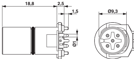
M12 male connector contact carrier
