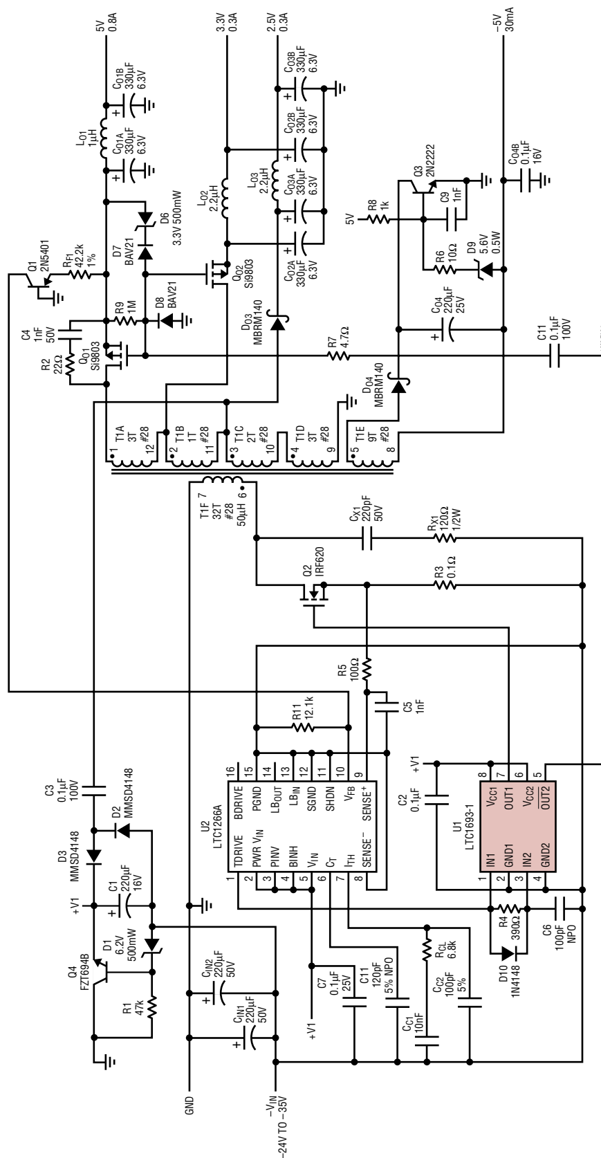
T1 WINDING ORDER: 1. T1A, T1B, T1C, D QUAD-FILAR, WOUND FIRST 2. AFTER A, T1B, T1C AND T1D, WOUND REMOVE 2 TURNS FROM T1B AND 1 TURN FROM T1C 1. T1E WOUND ON TOP, SPREAD EVENLY 2. LAYER OF INSULATION 3. T1F WOUND ON TOP, SPREAD EVENLY 4. T1F WOUND ON TOP, SPREAD EVENLY T1 CODE: COLTRONICS VP4-TYPE, AIR GAP, 0.7mm or 2 × 0.35mm SPACERS PRIMARY INDUCTANCE OF T1F = 50μH ALTERNATIVE CODES: SIEMENS EPD20, N67 MATERIAL, TDK PC40-EPG17
