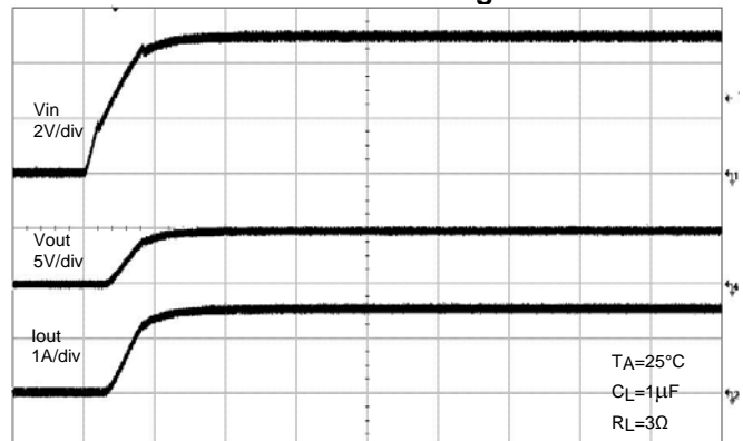
UVLO Increasing
