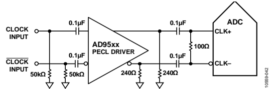
Figure 46. Differential PECL Sample Clock (Up to 625 MHz)
