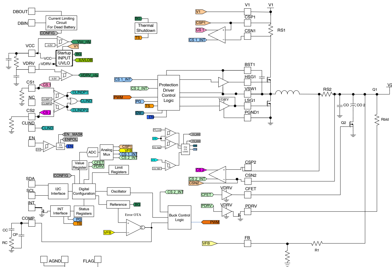
Figure 4. Block Diagram
