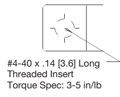
Threaded Mounting Flange 46XX-XXX5 Detail A
