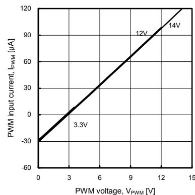
Figure 3. PWM Input Current
