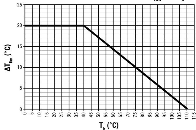
Maximum Overtemperature \Delta T_{lim} vs. T_h
