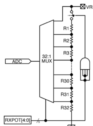
Figure 4. RXPOT Block Diagram
