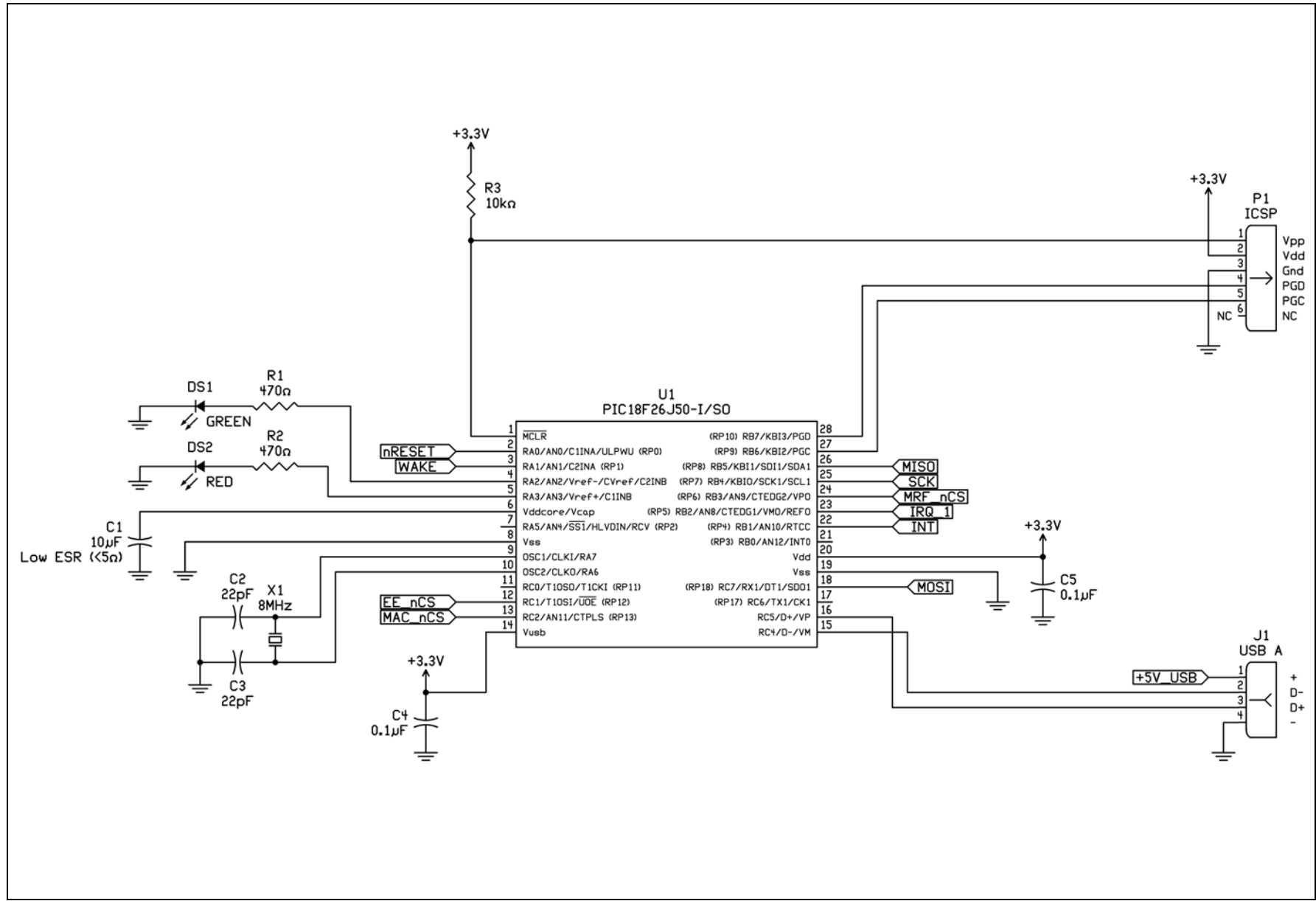
FIGURE A-1: ZENA™ WIRELESS ADAPTER SCHEMATIC
