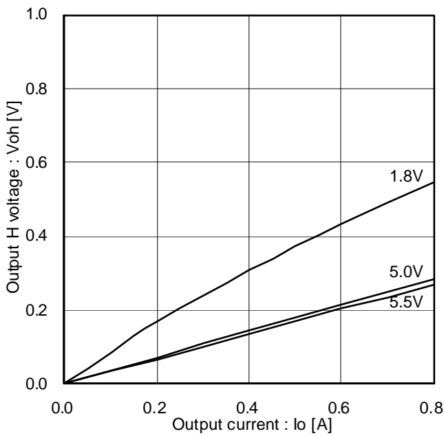
Figure 9. Output H voltage (Voltage characteristics)
