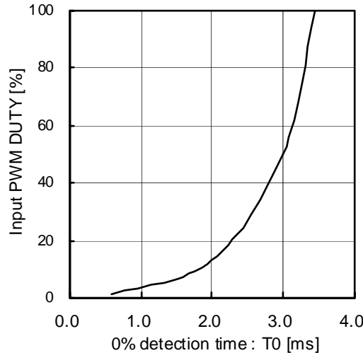
Figure 24. Characteristic 0% detection time and input PWM duty at 25kHz
