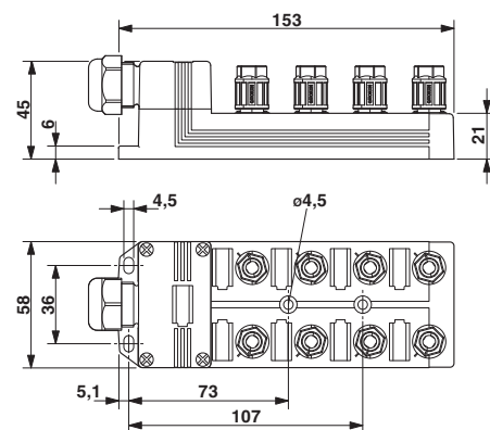
Dimensioned drawing
