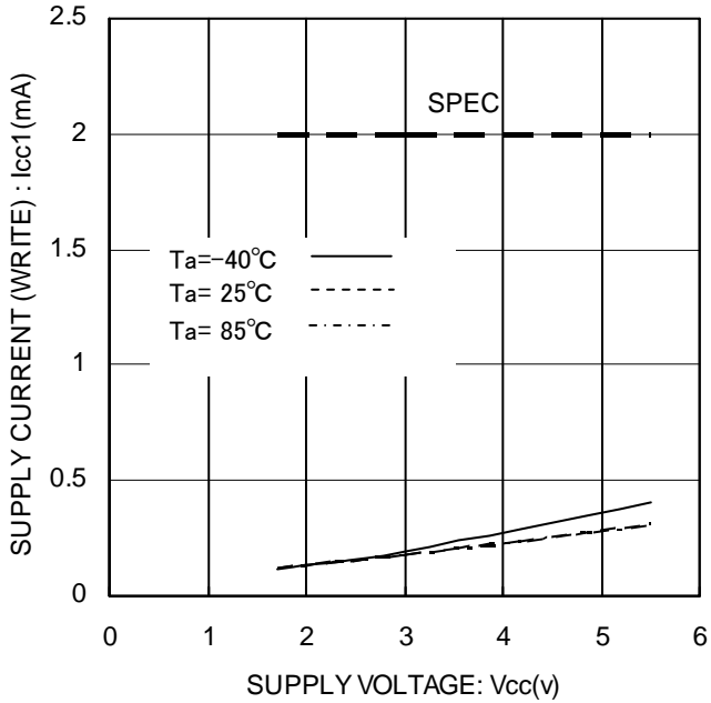
Figure 10. Supply Current (WRITE) I CC1 (f scl =1MHz)
