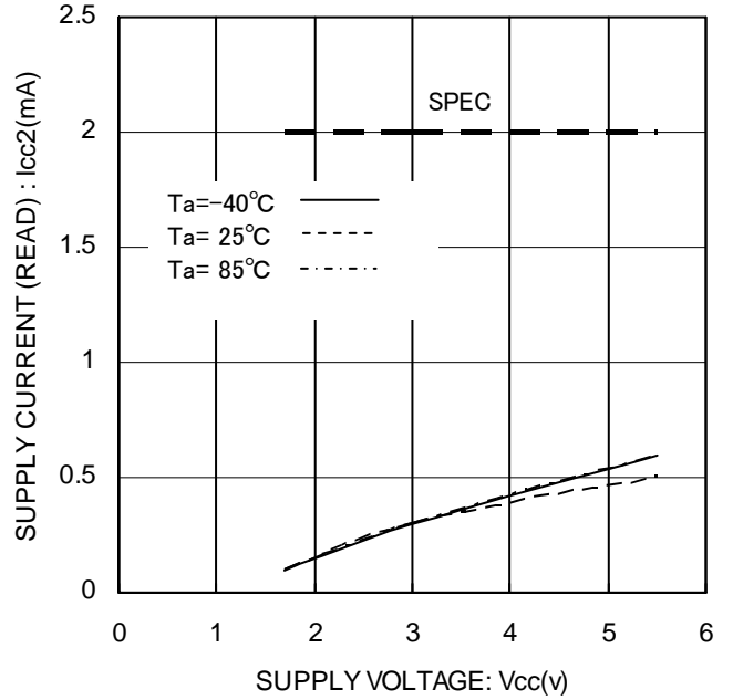
Figure 11. Supply Current (READ) I CC2 (f scl =1MHz)
