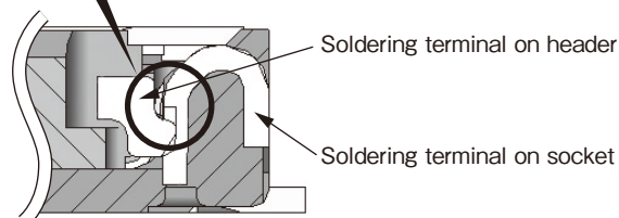
Cross section showing mating with soldering terminals
