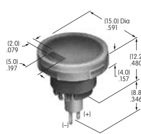
AT3011 Round Spot Illuminated Cap with Built-in LED Without Resistor; Volts: 2 With Resistor; Volts: 5 12 24 Polycarbonate Cap Colors: JA JB JC JE JF LED Colors: C D F CF Series: YB
