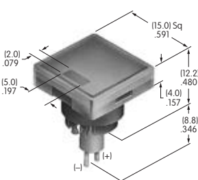
AT3010 Square Spot Illuminated Cap with Built-in LED Without Resistor; Volts: 2 With Resistor; Volts: 5 12 24 Polycarbonate Cap Colors: JA JB JC JE JF LED Colors: C D F CF Series: YB
