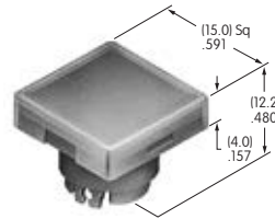
AT3004 Square Cap for Bright LED & Bicolor Polycarbonate Colors: JB JC JD JF Series: YB
