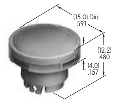
AT3005 Round Cap for Bright LED & Bicolor Polycarbonate Colors: JB JC JD JF Series: YB
