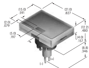
AT3012 Rectangular Spot Illuminated Cap with Built-in LED Without Resistor; Volts: 2 With Resistor; Volts: 5 12 24 Polycarbonate Cap Colors: JA JB JC JE JF LED Colors: C D F CF Series: YB
