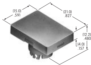
AT3010 Square Spot Illuminated Cap with Built-in LED Without Resistor; Volts: 2 With Resistor; Volts: 5 12 24 Polycarbonate Cap Colors: JA JB JC JE JF LED Colors: C D F CF Series: YB
