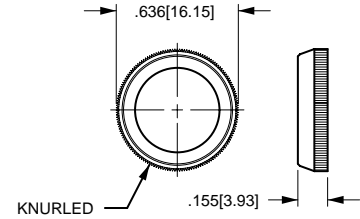
"DRESS" FACNUT .636" X .155" [16.15] X [3.93] NICKEL - 380-08810 BLACK - 380-08811
