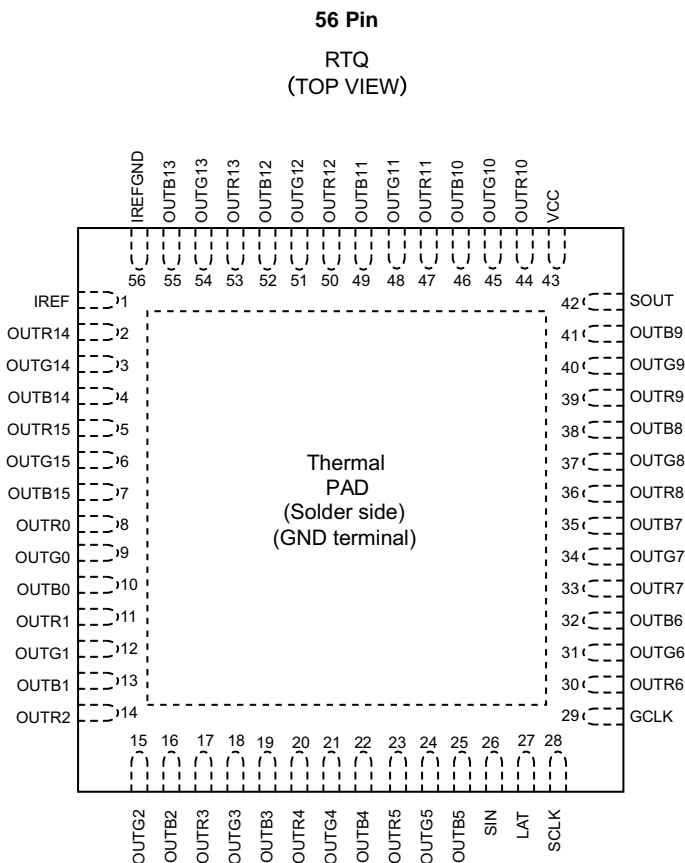
Pin Functions
