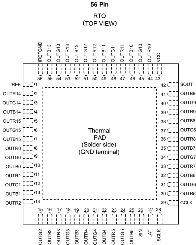
Pin Functions
