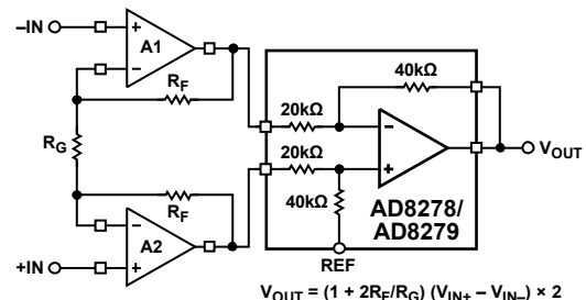
Figure 60. Low Power Precision Instrumentation Amplifier
