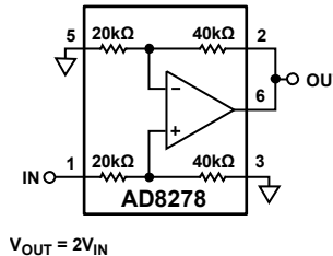
Figure 57. Noninverting Amplifier, Gain = 2
