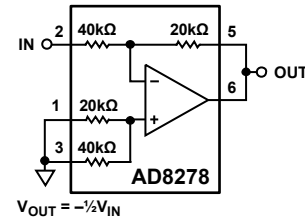
Figure 55. Inverting Amplifier, Gain = -1/2
