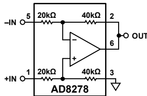
Figure 52. Difference Amplifier, Gain = 2
