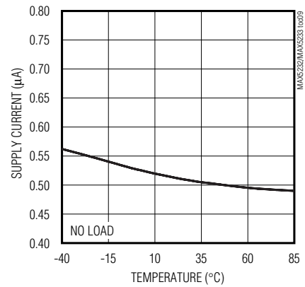
FULL POWER-DOWN SUPPLY CURRENT vs. TEMPERATURE (MAX5233)
