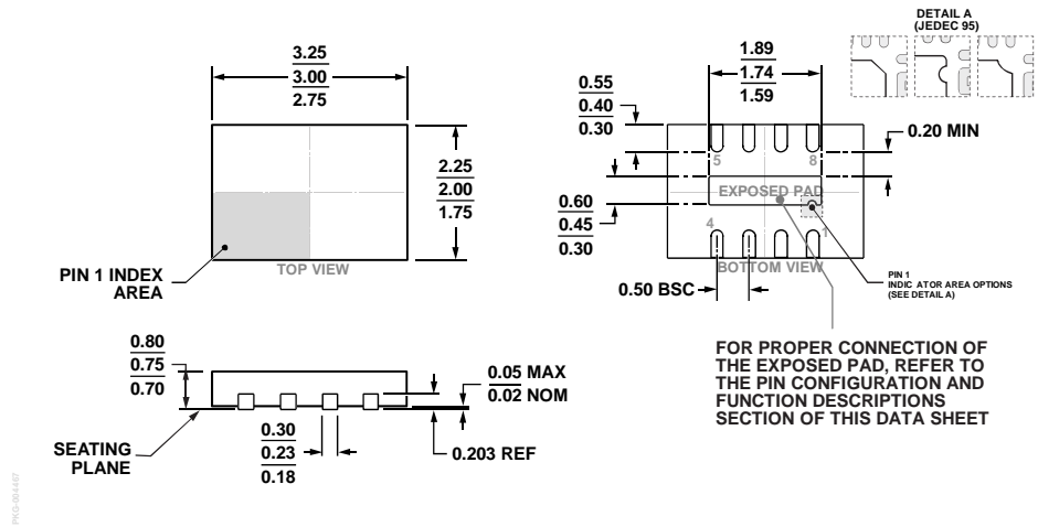
Figure 44. 8-Lead Lead Frame Chip Scale Package [LFCSP] 2 mm x 3 mm Body and 0.75 mm Package Height (CP-8-23) Dimensions shown in millimeters
