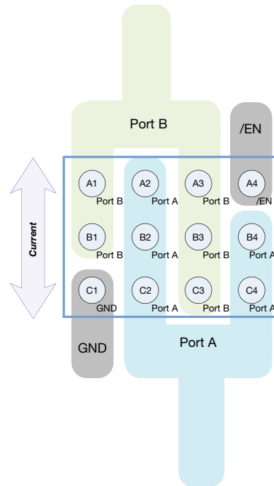
Fig. 18 - Proposed Layout
