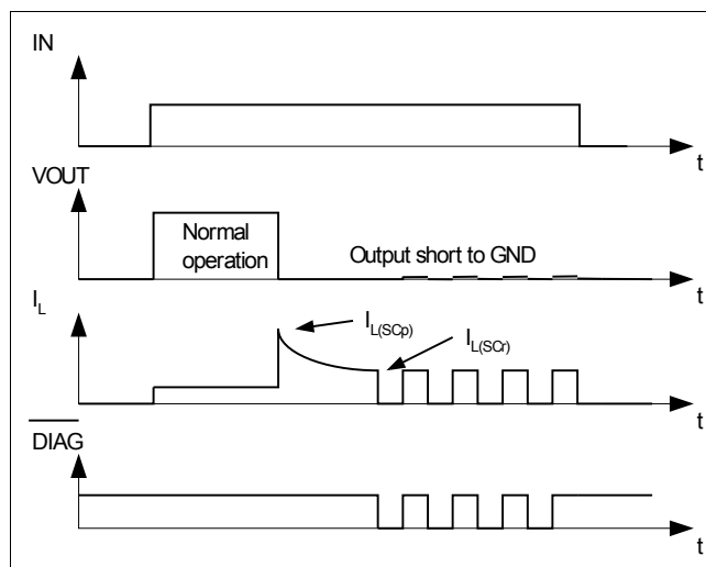
Figure 7 Short circuit in on-state, shut down by overtemperature, restart by cooling
