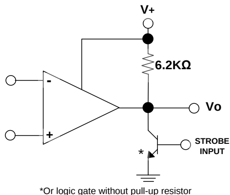
Output Strobing
