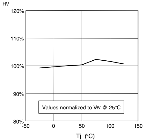
Figure 9. High-voltage generator V cc restart voltage vs. Tj
