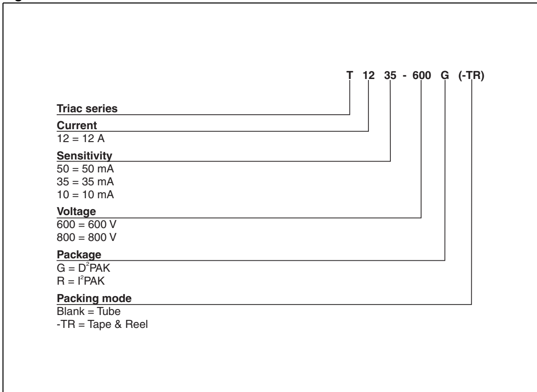
Figure 14. T12xx series
