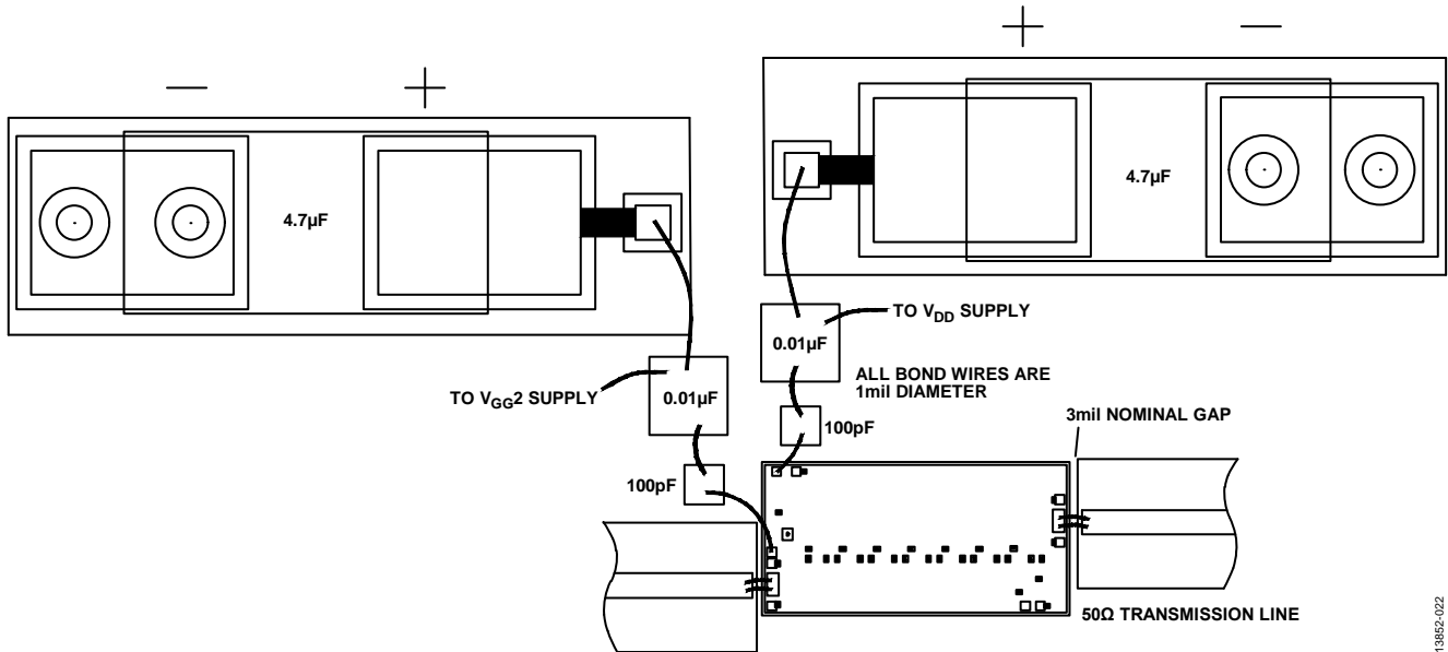
Figure 37. Assembly Diagram
