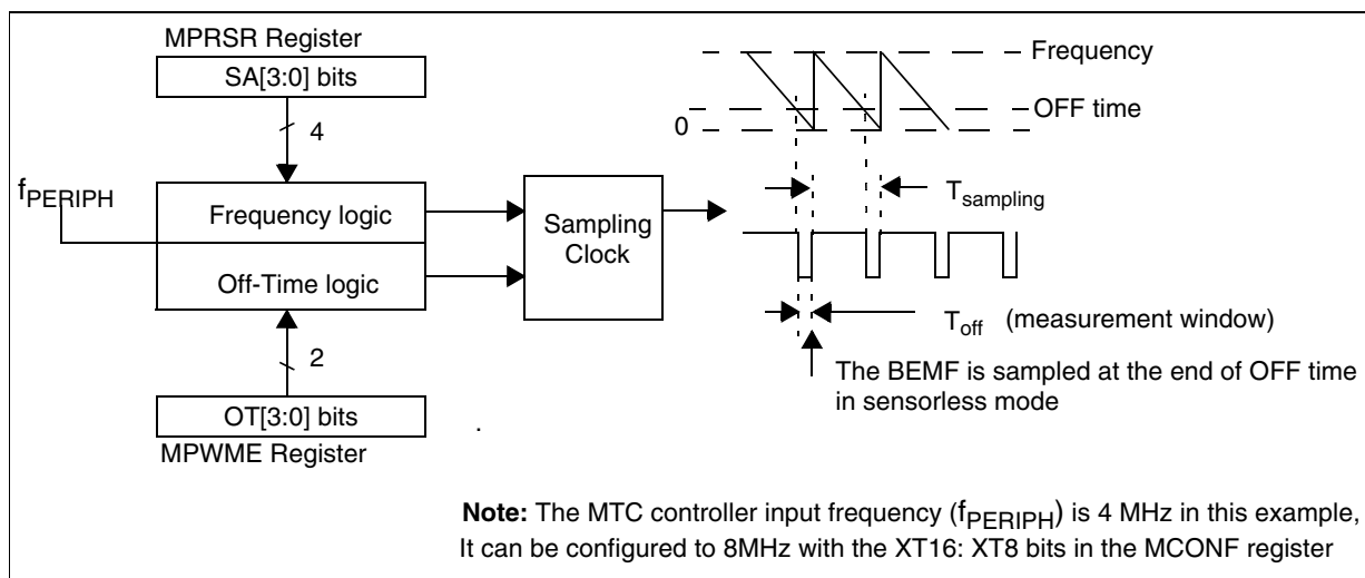
Figure 107. Sampling clock generation block
