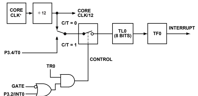
Figure 78. Timer/Counter 0, Mode 3
