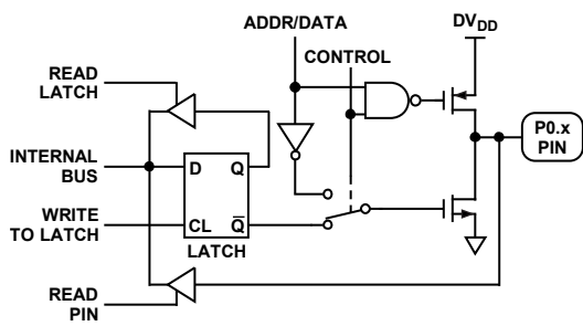
Figure 66. Port 0 Bit Latch and I/O Buffer
