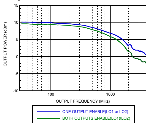
Figure 11. Differential Output Power (LO1, LO2) [8] [9]
