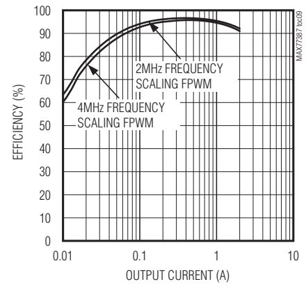
DC-DC CONVERTER EFFICIENCY vs. LOAD CURRENT ( V_{IN} = 3.7V , V_{OUT} = 4V ) 1\mu H
