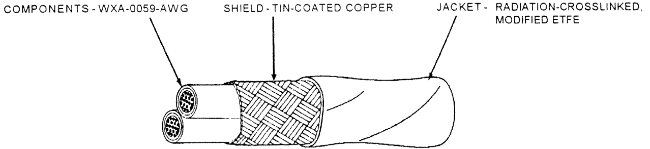
EXAMPLE: CXA-0078-24-2 (TWO CONDUCTOR CABLE)
