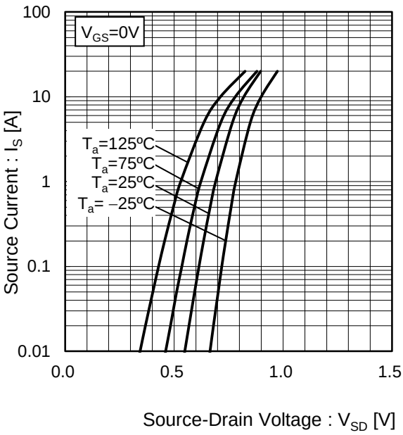
Fig.22 Source Current vs. Source - Drain Voltage
