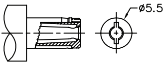
MATING PLUG Jack Insertion Depth: 8.5 mm
