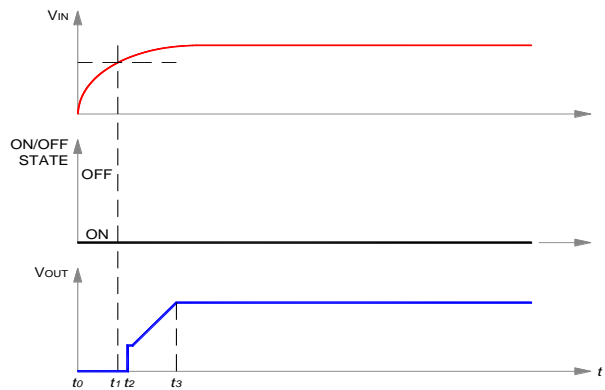
Figure 5. Start-up scenario #1.
