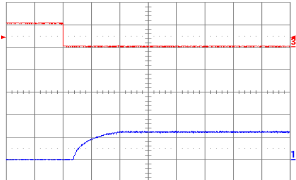
Figure 1.2V.16. Turn-on transient at full rated load current (resistive) plus 10,000 \mu\text{F} at V_{in} = 48\text{ V} , triggered via ON/OFF pin. Top trace: ON/OFF signal (5 V/div.). Bottom trace: output voltage (1 V/div.). Time scale: 2 ms/div.
