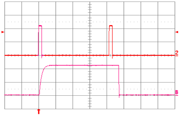
Figure 2.5V.24. Load current (top trace, 20 A/div., 50 ms/div.) into a 10 m \Omega short circuit during restart, at V_{in} = 48 \text{ V} . Bottom trace (20 A/div., 2 ms/div.) is an expansion of the on-time portion of the top trace.
