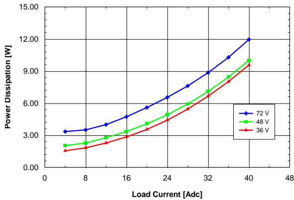
Figure 1.0V.13. Power dissipation vs. load current and input voltage for QME48T40010 converter mounted horizontally with air flowing from pin 1 to pin 3 at a rate of 300 LFM (1.5 m/s) and T_a = 25\text{ }^\circ\text{C} .
