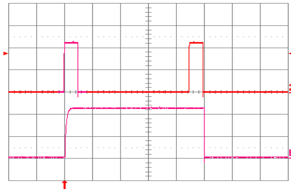
Figure 1.0V.24. Load current (top trace, 20 \text{ A}/\text{div} ., 50 \text{ ms}/\text{div} .) into a 10 \text{ m}\Omega short circuit during restart, at V_{in} = 48 \text{ V} . Bottom trace ( 20 \text{ A}/\text{div} ., 5 \text{ ms}/\text{div} .) is an expansion of the on-time portion of the top trace.
