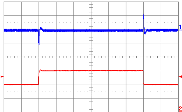
Figure 1.2V.18. Output voltage response to load current step-change (20 A - 30 A - 20 A) at V_{in} = 48\text{ V} . Top trace: output voltage (100 mV/div.). Bottom trace: load current (10 A/div.). Current slew rate: 5 A/ \mu\text{s} . C_o = 470\ \mu\text{F} POS + 1 \mu\text{F} ceramic. Time scale: 0.2 ms/div.
