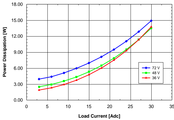
Figure 3.3V.13. Power dissipation vs. load current and input voltage for QME48T40033 converter mounted horizontally with air flowing from pin 1 to pin 3 at a rate of 300 LFM (1.5 m/s) and T_a = 25^\circ\text{C} .
